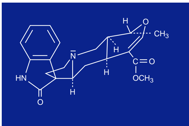
Figure 1. Structure of Isopteropodine
